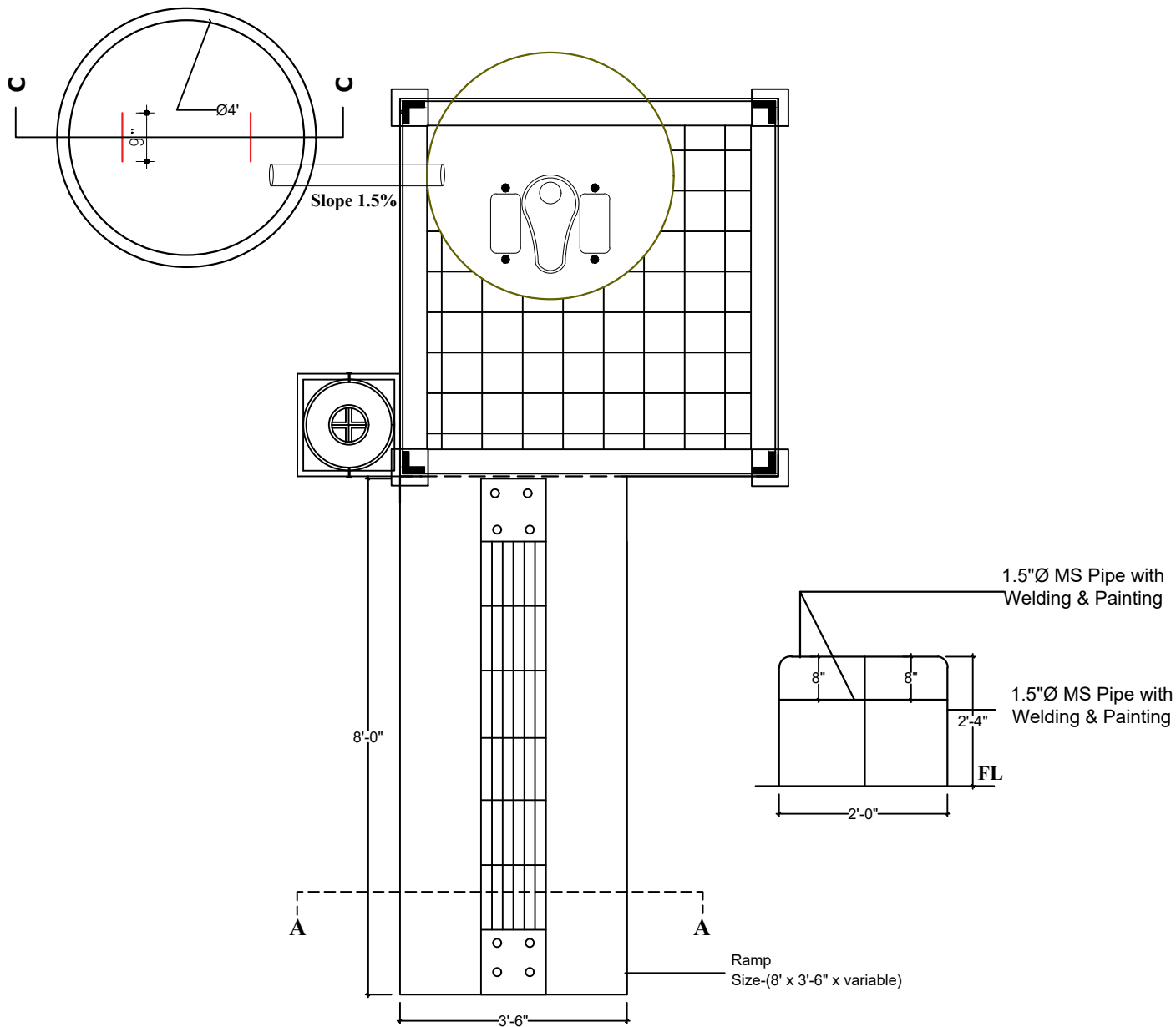
PLAN OF LATRINE WITH TWIN PIT (STEEL FRAME)
