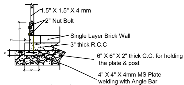
Section P: Joint Section
