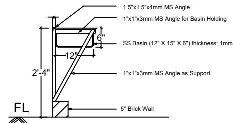
SIDE ELEVATION OF SS BASIN
