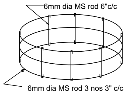
Rod placement for Ring
