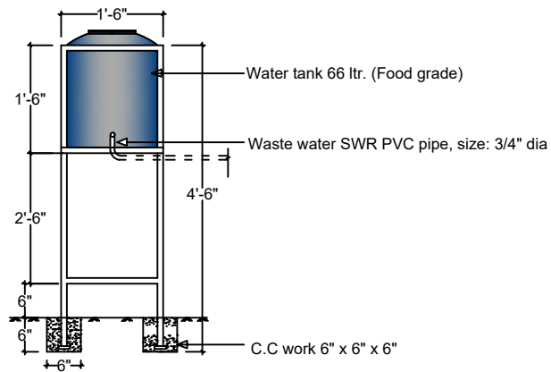
FRONT ELEVATION WATER TANK
