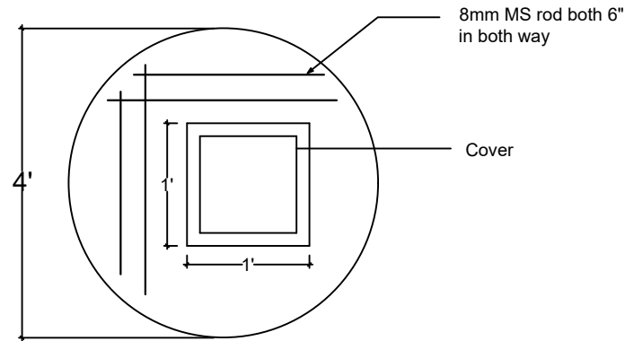
Rod placement for cover slab
