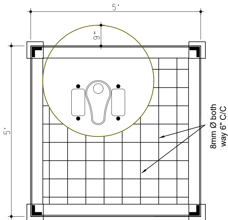
Section: Reinforcement Details of Slab
